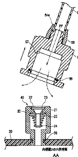
AA Internal space of endoscope 2
